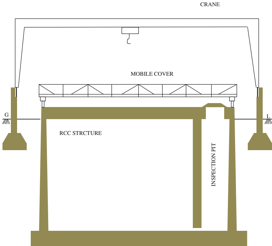
Fig. 10.10 Concrete trench for disposal of radioactive waste
